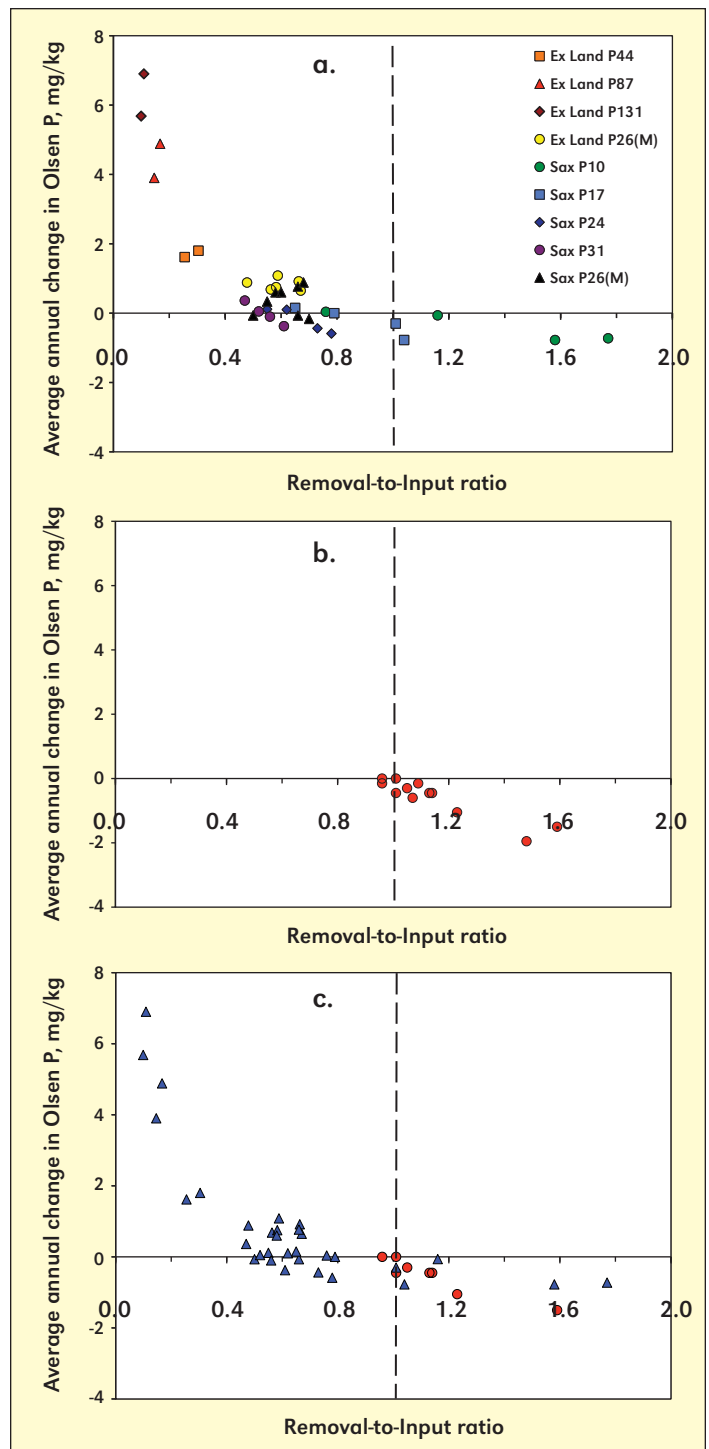
Figure 2. Relationship between the removal-to-input ratio (P removed by the crop divided by fertilizer P inputs) and the change in plant-available P for (a) two long-term experiments in the U.K. [P44 etc. denotes average annual application of fertilizer P; (M) denotes a maintenance dressing]; (b) 12 states in the U.S. (P Fixen, Pers. Comm.); (c) all U.S. ●, and U.K. ▲, data.
