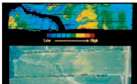
Figure 5. EM-38 sensor readings (top) and aerial corn crop cover photo (July 25, 1997) at Centralia, Missouri site.
