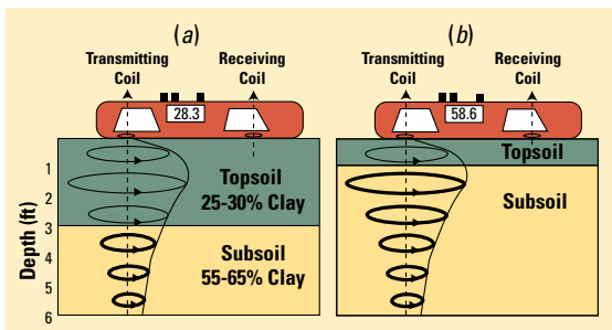
Figure 1. EM-38 principle of operation in soils.
