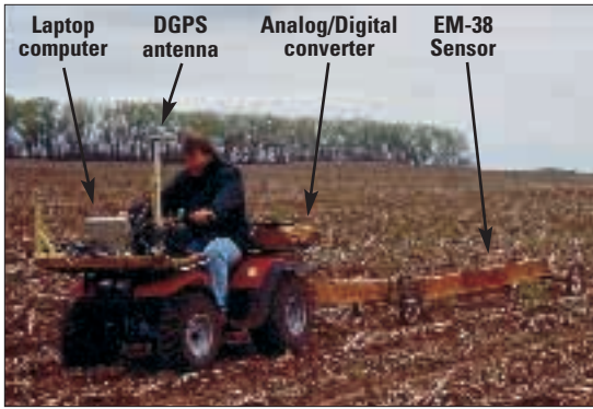
Figure 2. Mobile EM-38 sensor unit is pulled behind a four-wheel ATV, equipped with analog/digital converter, laptop computer, and DGPS antenna.
