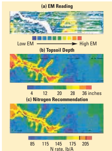
Figure 4. EM-38 soil conductivity, topsoil depth, and N recommended for corn at Centralia, Missouri.
