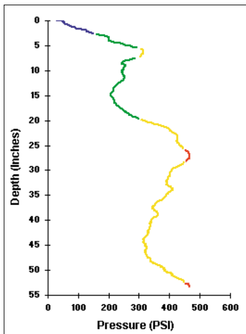
Figure 2. Compaction profile created from a penetrometer. Compaction categories are delineated by color (light=blue, medium=green, high=yellow, heavy=red).
