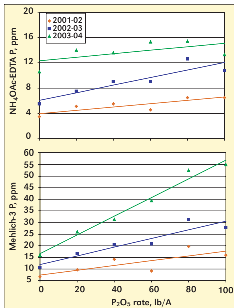
Figure 3. Soil P levels from two methods of extraction after the 2002, 2003, and 2004 growing seasons at Stephenville, Texas.
