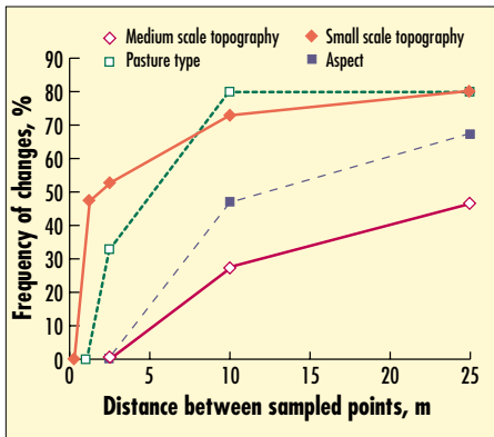
Figure 2. At the smallest sampling distance of 0.25 m, no changes occurred in any of the descriptive landscape categories.
